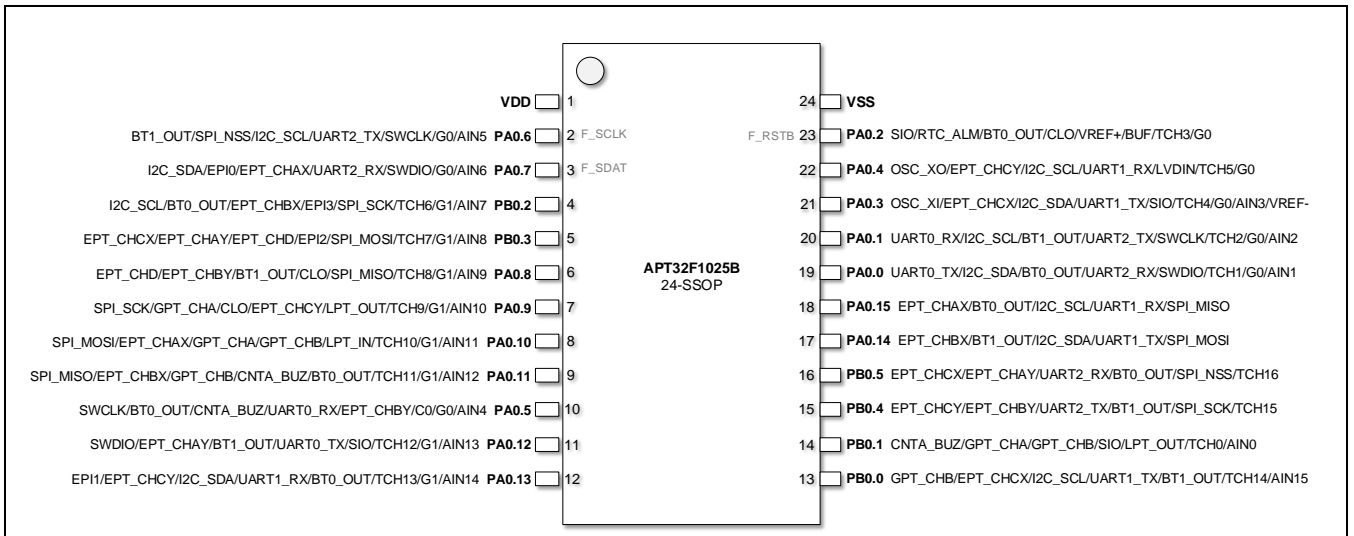
Figure 2-1 管脚定义图(24PIN)
