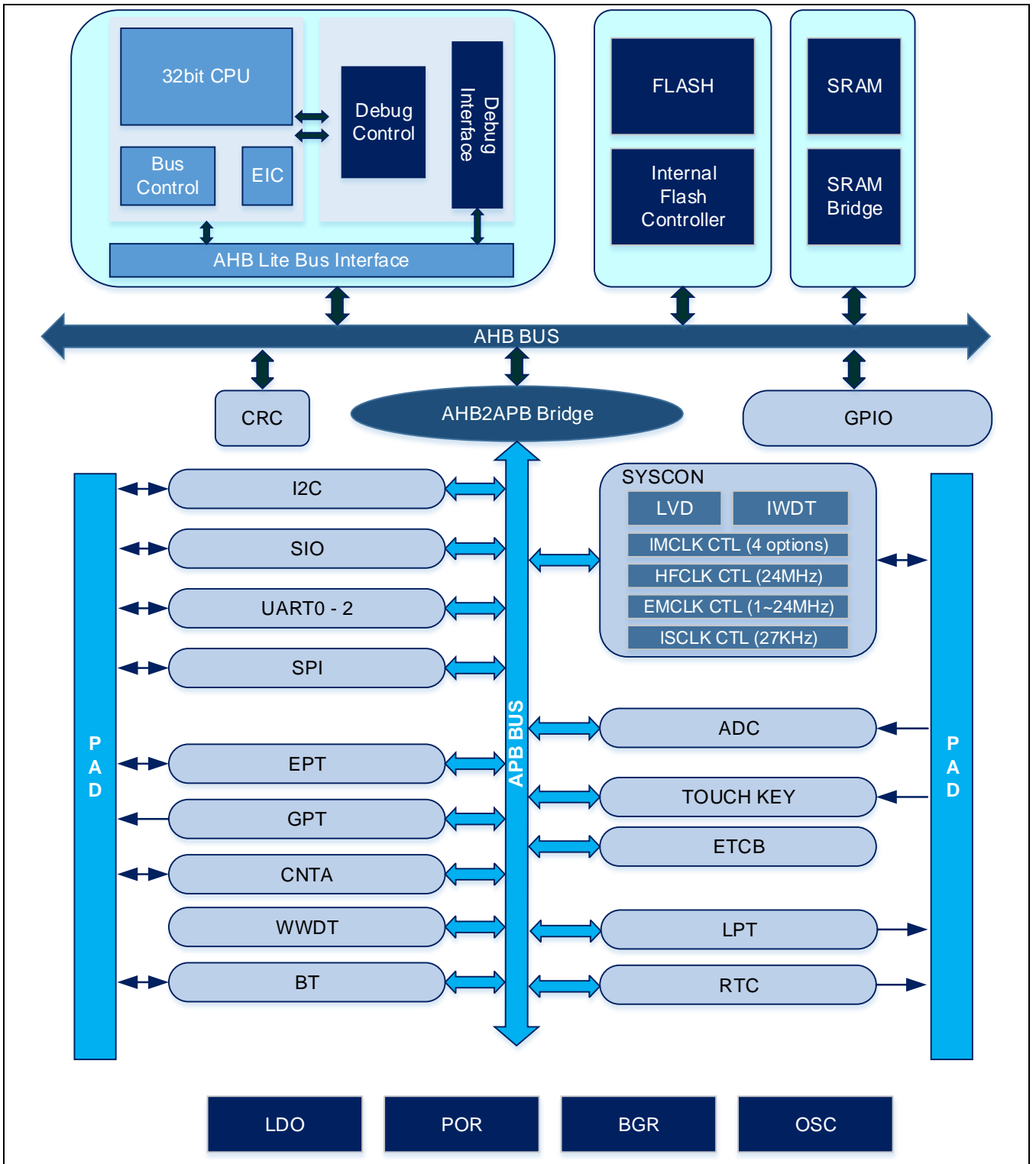
Figure 1-1 APT32F1025B模块框图
