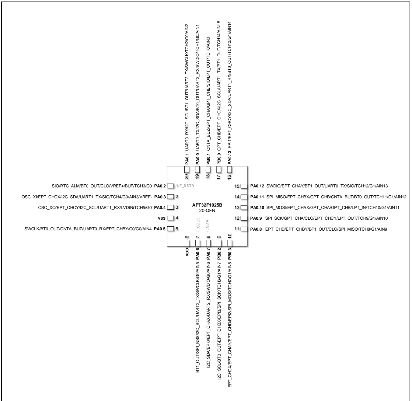
Figure 2-2 管脚定义图(20QFN)
