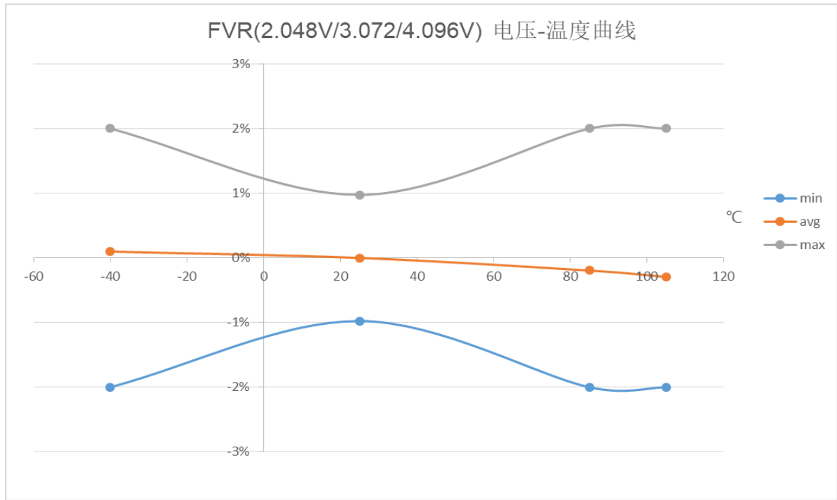
Figure 3-14 FVR电压温度曲线
