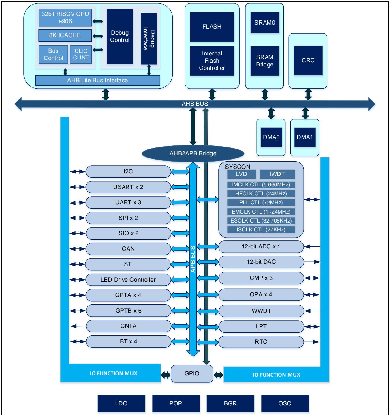
Figure 1-1 APT32F1731模块框图
